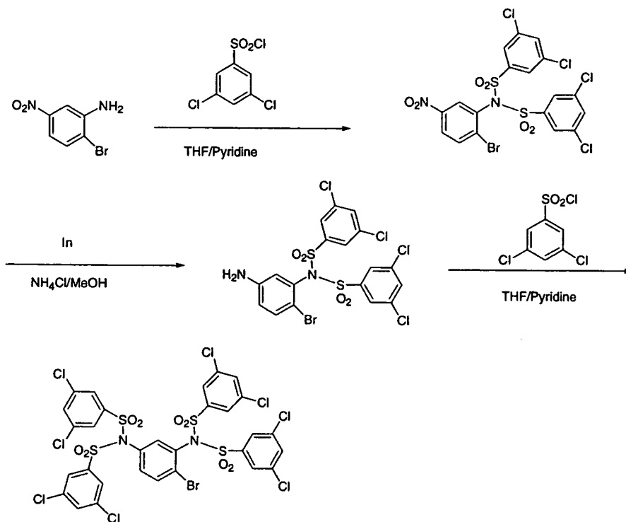
Scheme IV-B
